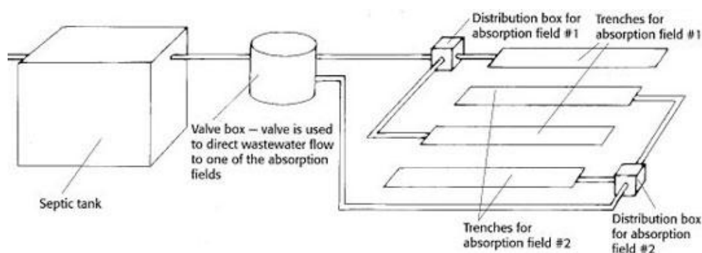
Figure 4.4 Septic systems with alternating trenches.
