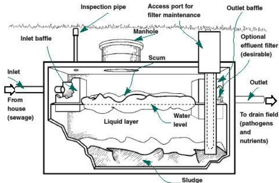
Figure 4.2 The parts of a septic tank.
